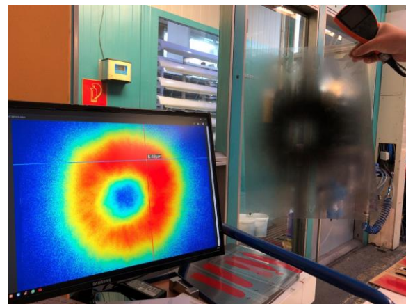
Figure 3: A Sprayed Foil and Its Captured Image Displayed in “Heat Map” Format
