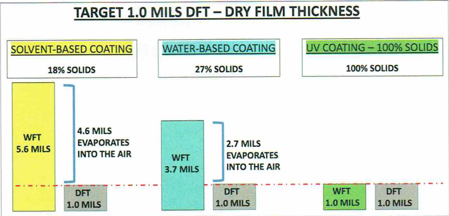
Figure 1. WFT = wet film thickness vs. DFT = dry film thickness
